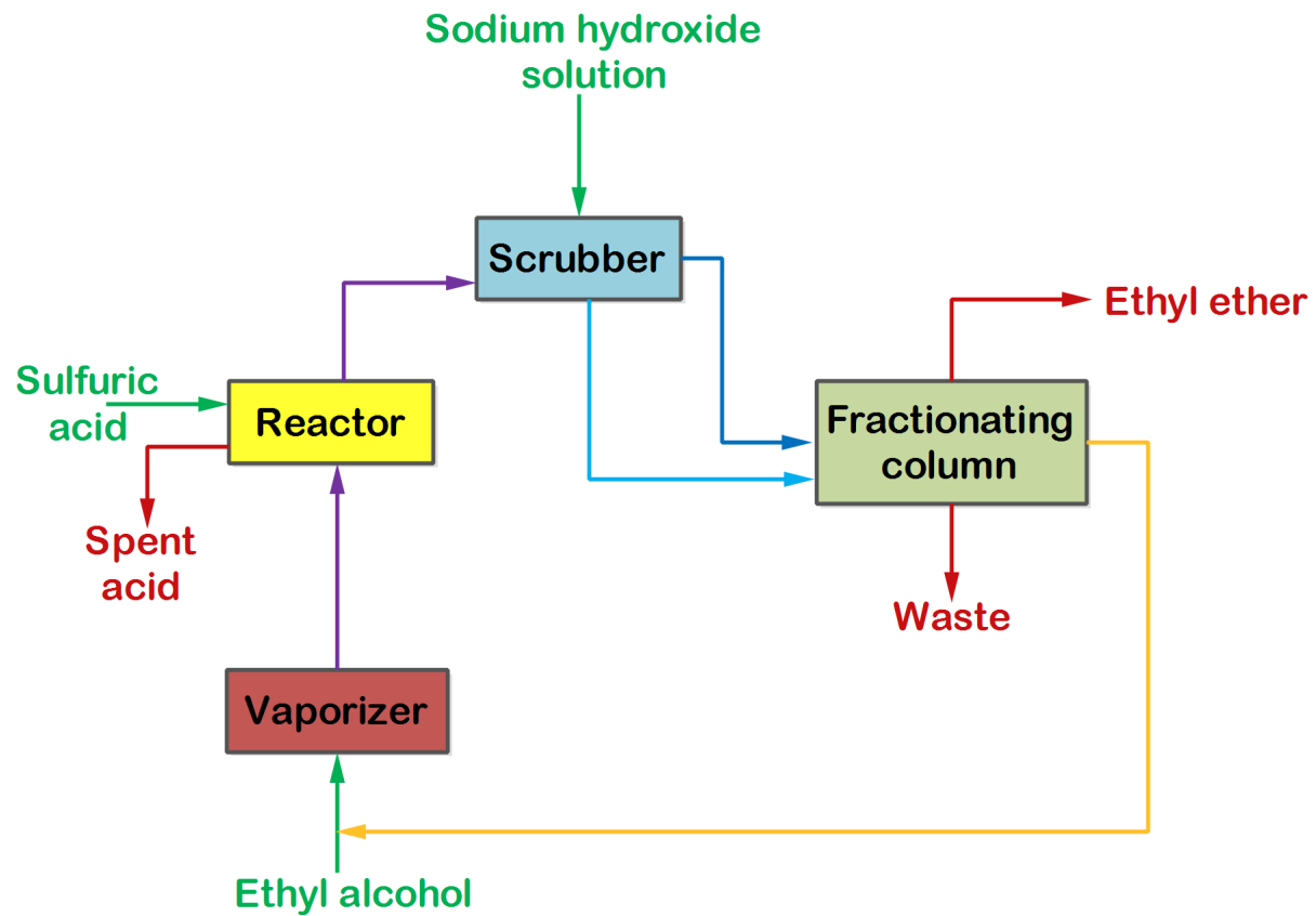
Figure: Manufacture of diethyl ether by dehydration of ethyl alcohol
